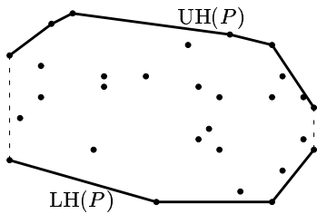
Fig. 1. The convex hull CH(P) of a set of points P can be partitioned into an upper hull UH(P) , a lower hull LH(P) , and possibly two vertical lines.
